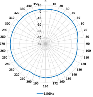
BLE/ZigBee 2.4GHz Band - Azimuth
