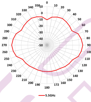
5.0GHz Band - Elevation
