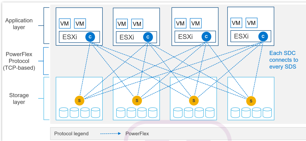
Example of SDC – SDS communication with SDC installed in ESXi.
